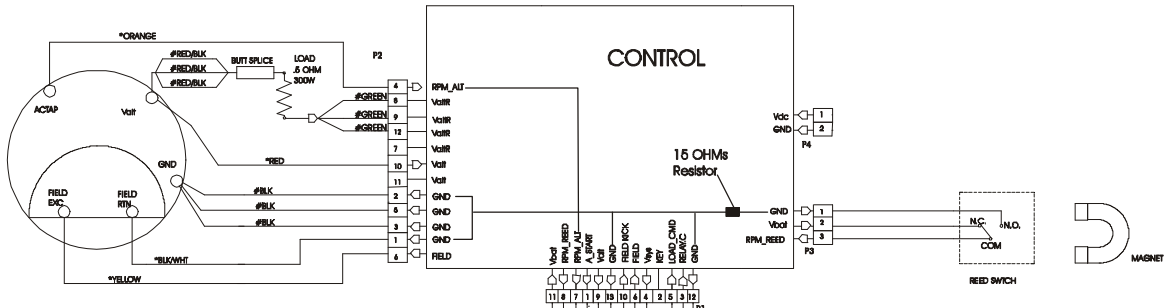
CABLE ASSEMBLY POWER CONTROL TO ALTERNATOR AK63-00029-0001
